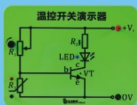
温控开关演示器 Temperature control switch demonstrator
