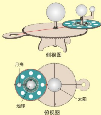
自制三球仪模型 Self-made three-sphere instrument model
