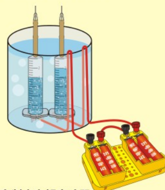
自制水电解实验器 Homemade water electrolysis experimental apparatus
