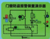
门窗防盗报警装置演示器 Door and window anti-theft alarm device demonstrator
